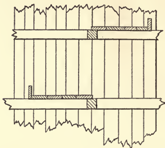
FIG. 12.—CROSS-STAGING IN TRENCH.
